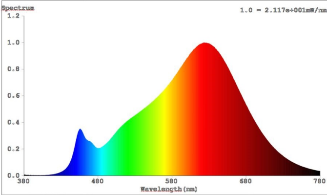
Spectral Distribution
