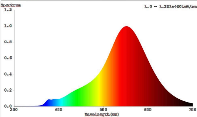
Spectral Distribution
