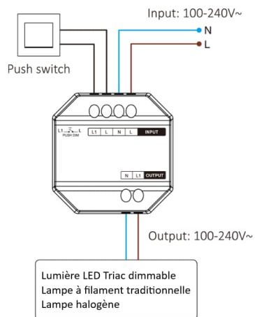
AC Triac Dimmer (TRI-C1)
